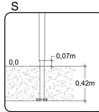
S Sunken Foundation 8113274
